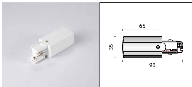
Live-end connector(Left)
