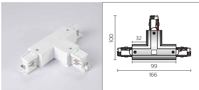
"T" connector(Right2)
