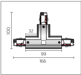
Twisted "T" connector(Right) (R1 can be changed into R2)
