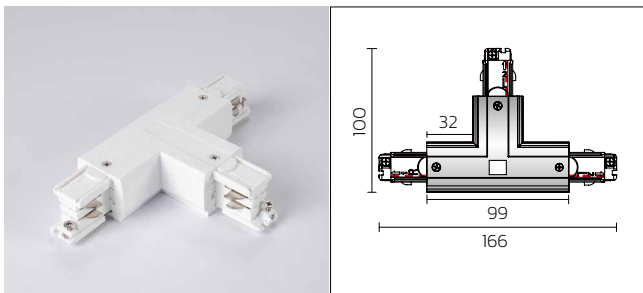
"T" connector(Right1)
