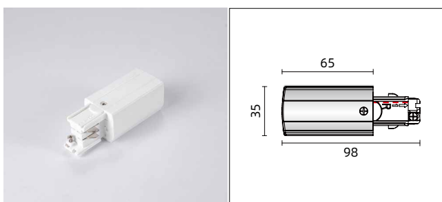
Live-end connector(Right)
