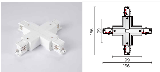
"+" connector
