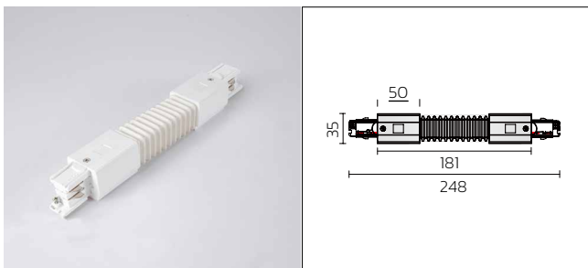
Flexible connector
