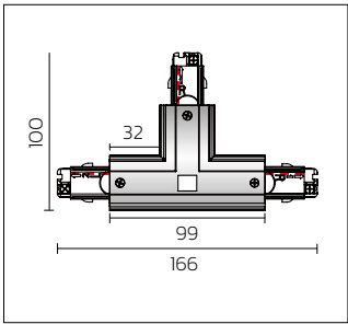
Twisted "T" connector(Left) (L1 can be changed into L2)
