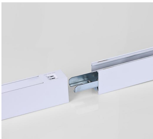
Step 2 Fasten LUS589-JOINER
