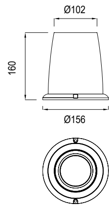
ATP168 GROUND MOUNTED
